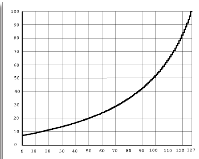
Maximum speed characteristic (see CV05 / par013) in shunting gear (see CV61 / par018)
